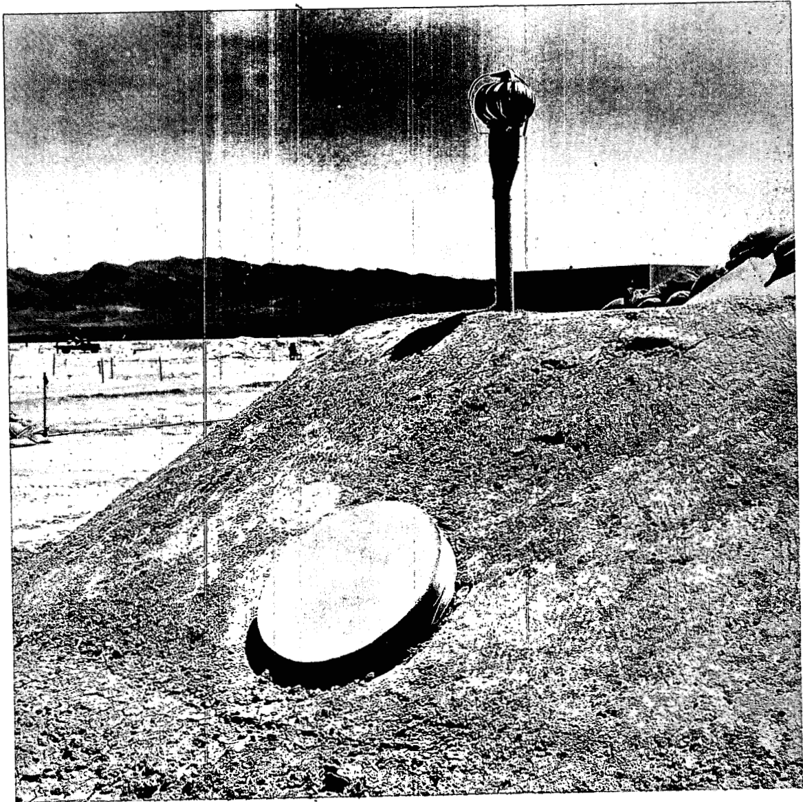
Fig. 5—Exhaust pipe with air-driven ventilator; escape hatch with cover in foreground.
